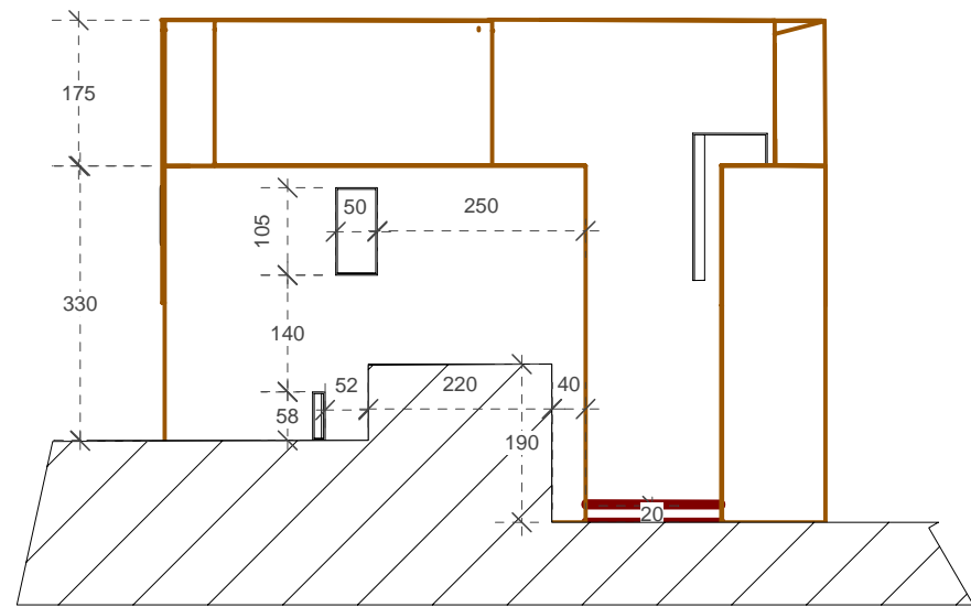
FACADE SUD
