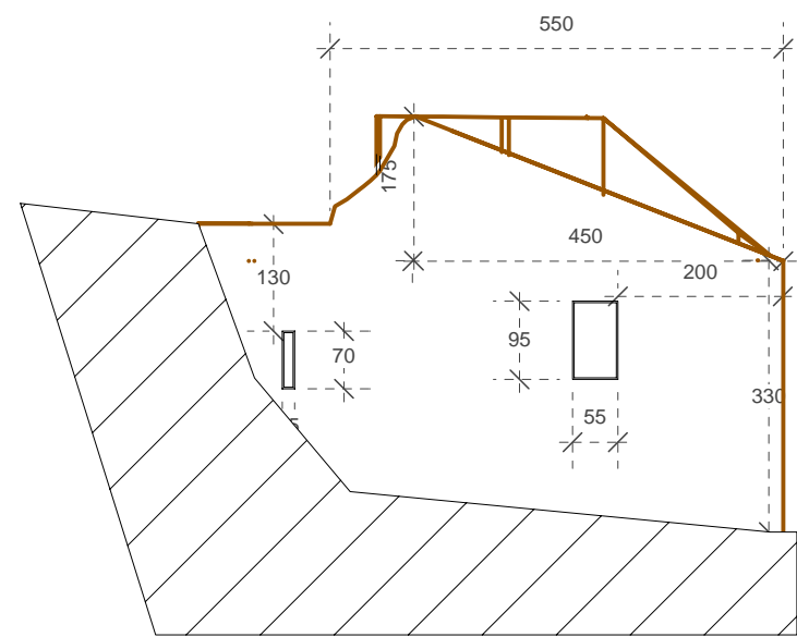
FACADE SUD
